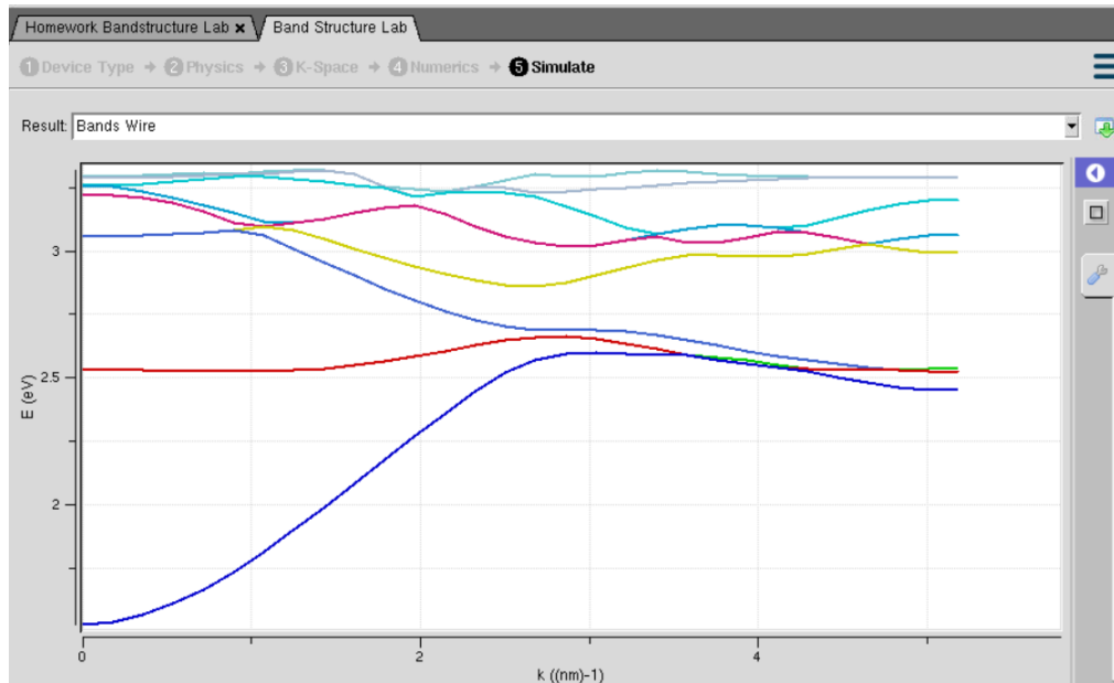
Fig 3: This figure shows the band structure of a semiconductor nanowire simulated using the NanoHub Band Structure Lab. The colored energy bands indicate how electron energy changes with the wave vector ( k ), revealing the electronic behavior of the material.
